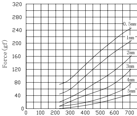
Ampere-turns (AT)
