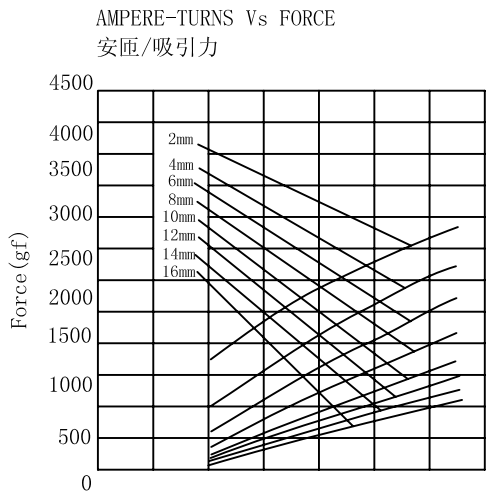
Ampere-turns (AT)
